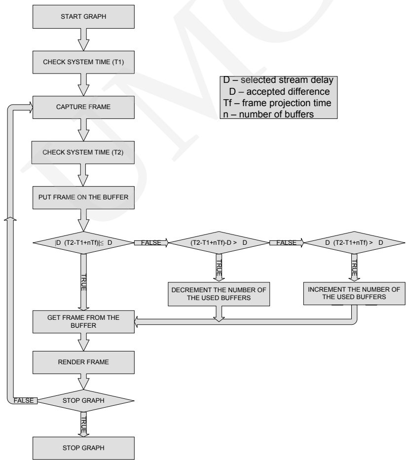
Fig. 4. The video delay algorithm in the “Kamera” program
