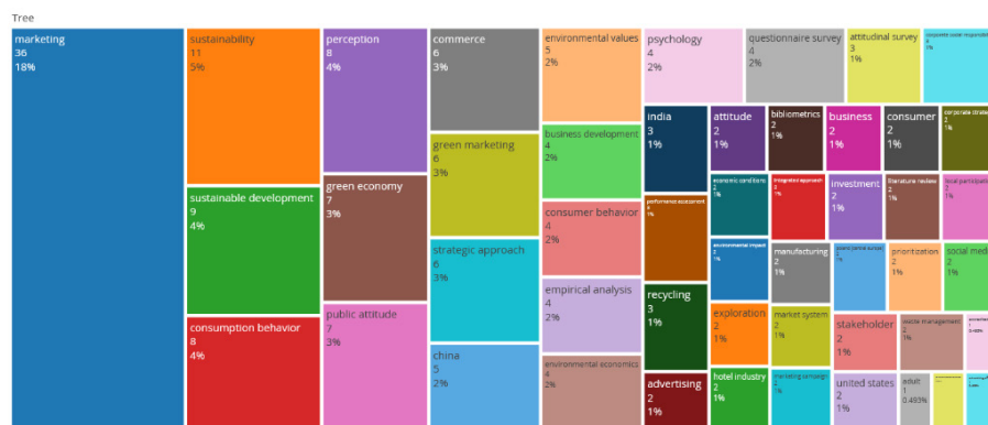
Figure 5. Tree map
